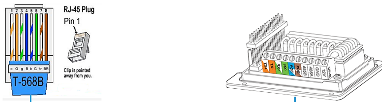
Figure 6: Connection Example
