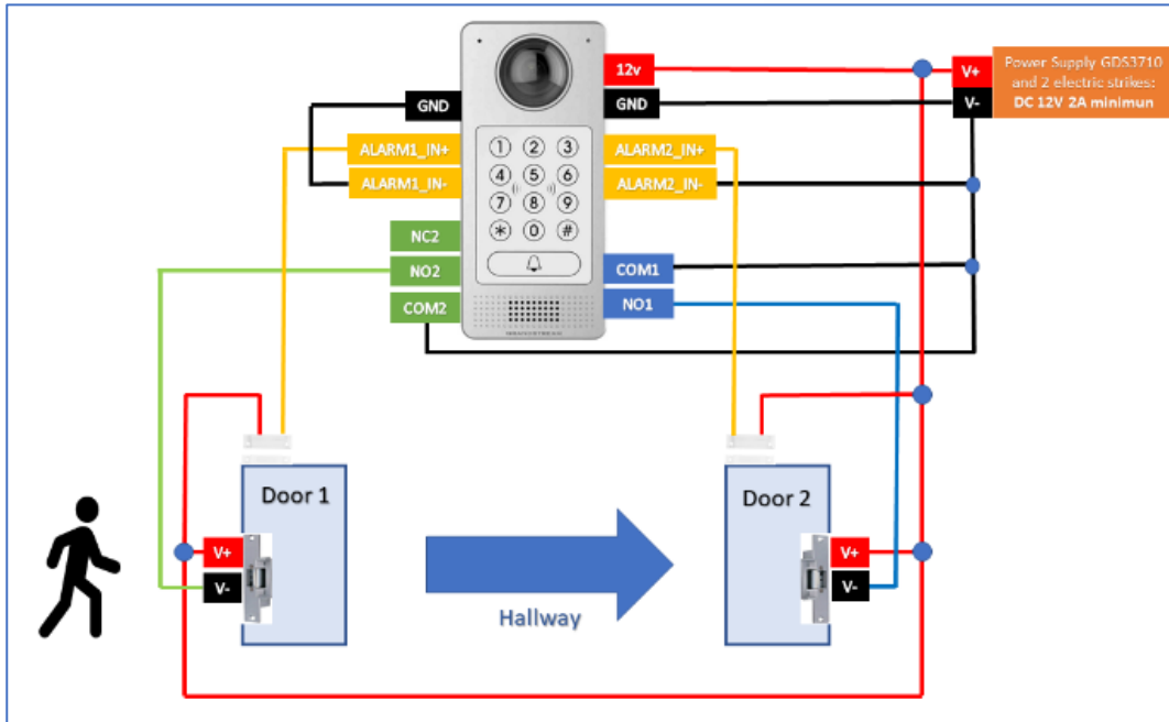
Figure 39: One-Way Interlocking Mode Diagram Example
