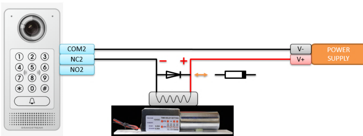
Electric lock
