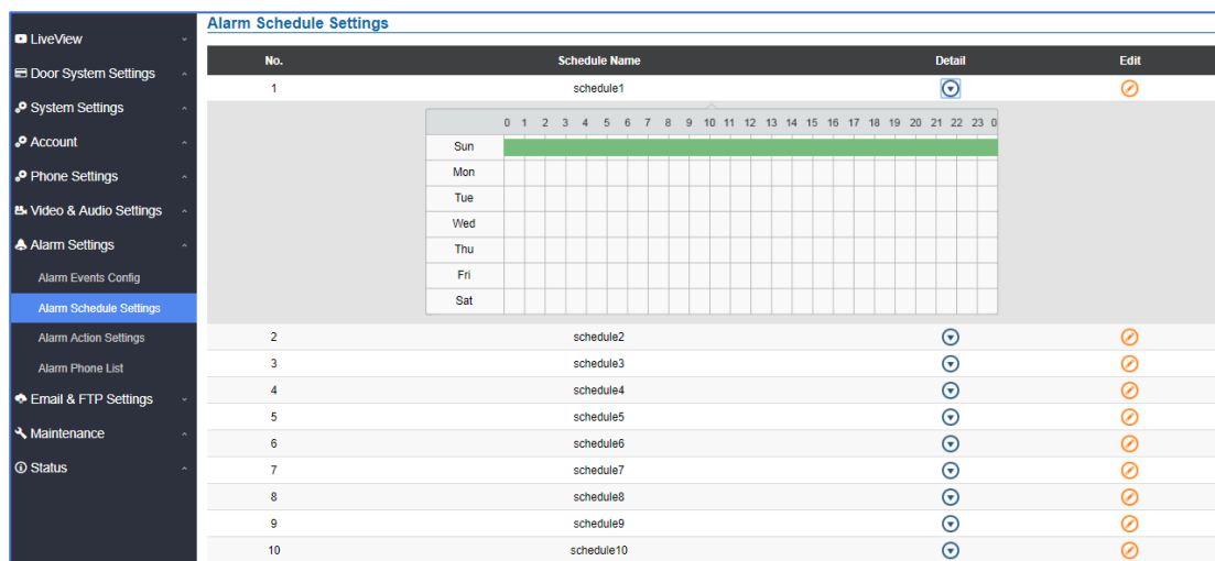
Figure 94: Alarm Schedule
