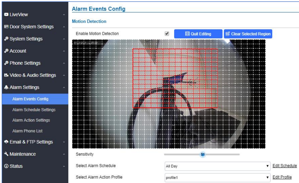
Figure 92: Region Config
