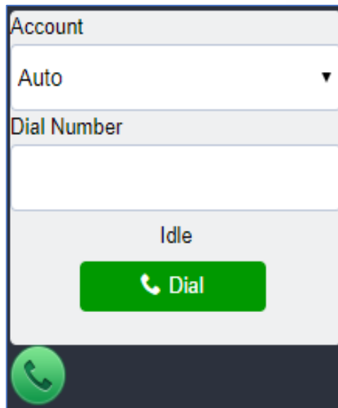
Figure 85 : Click-To-Dial
